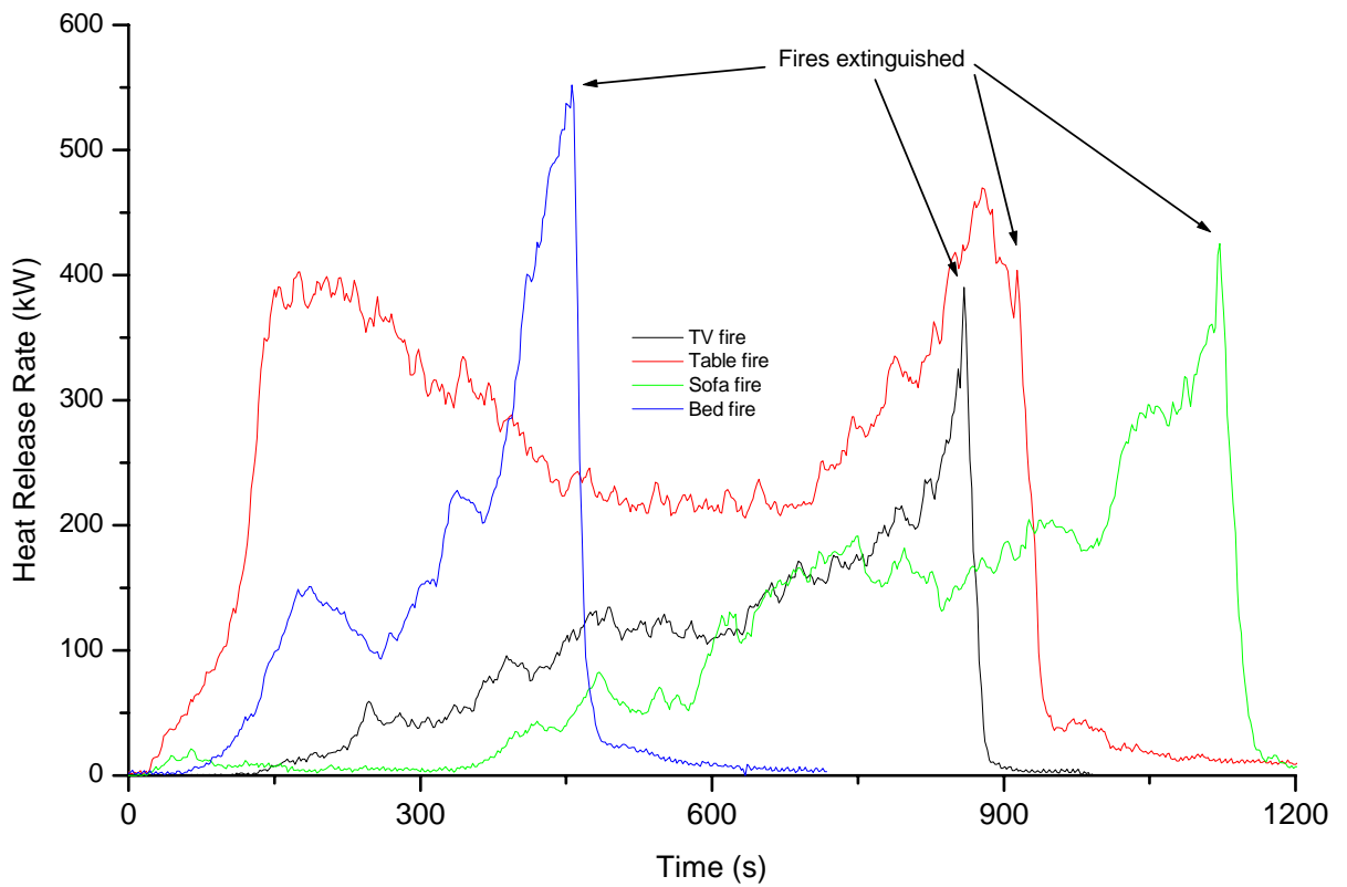
Figure 5I.5 – Comparison of heat release rate profiles
