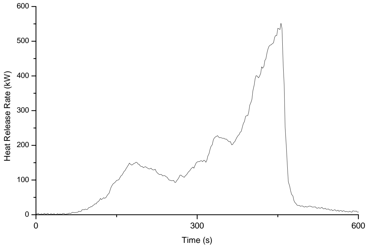
Figure 5I.4 – Bed profile for Sofa fire (test terminated after 7½ mins)
