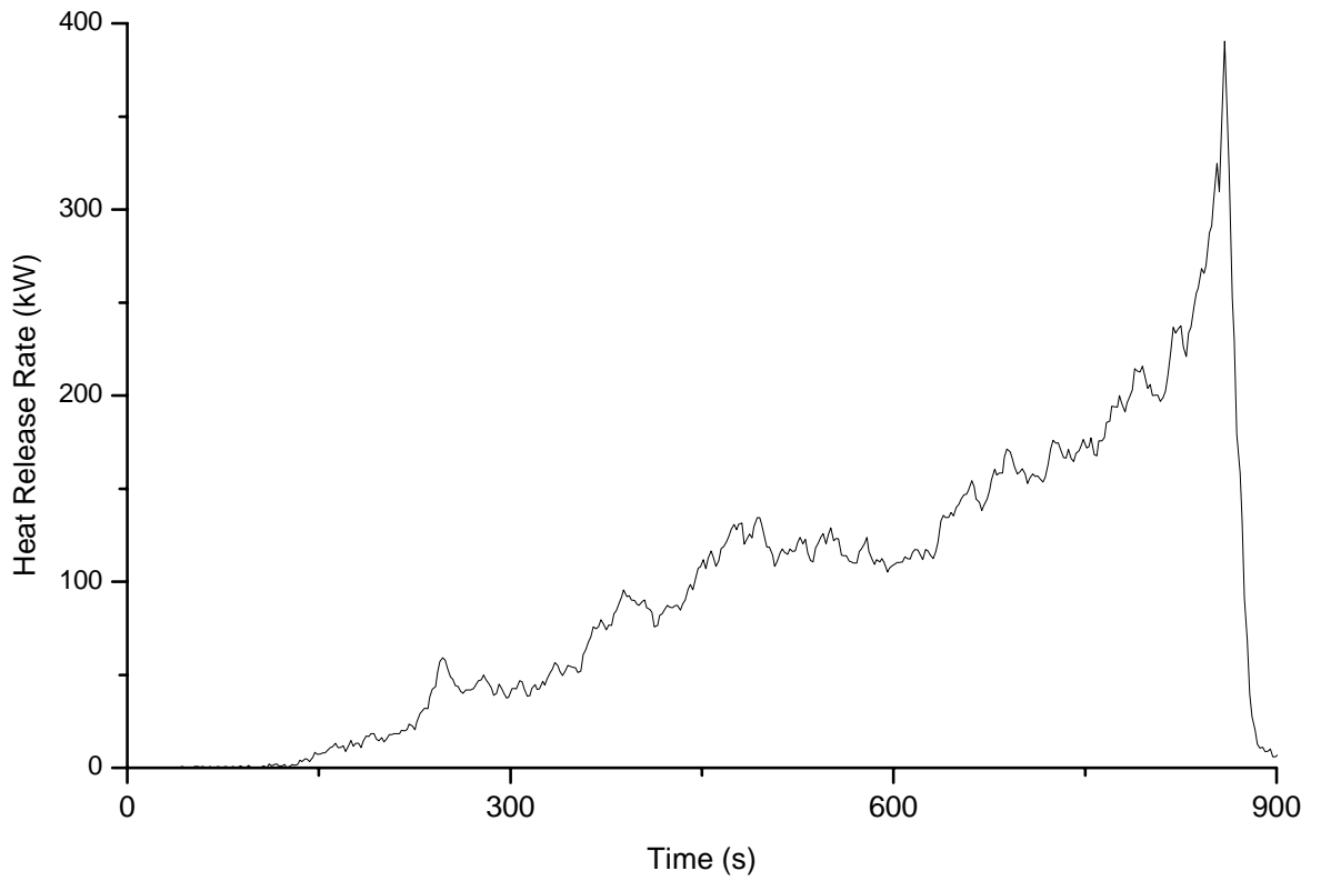
Figure 5I.1 – Heat Release Rate profile for TV fire (test terminated after 14 mins)
