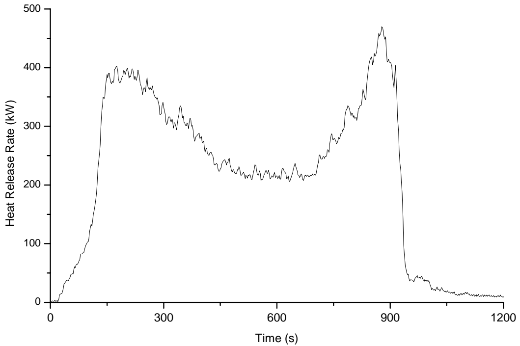
Figure 5I.2 – Heat Release Rate profile for Table fire (test terminated after 15 mins) – Moisture content of top table 12% and wooden batons 10.5%
