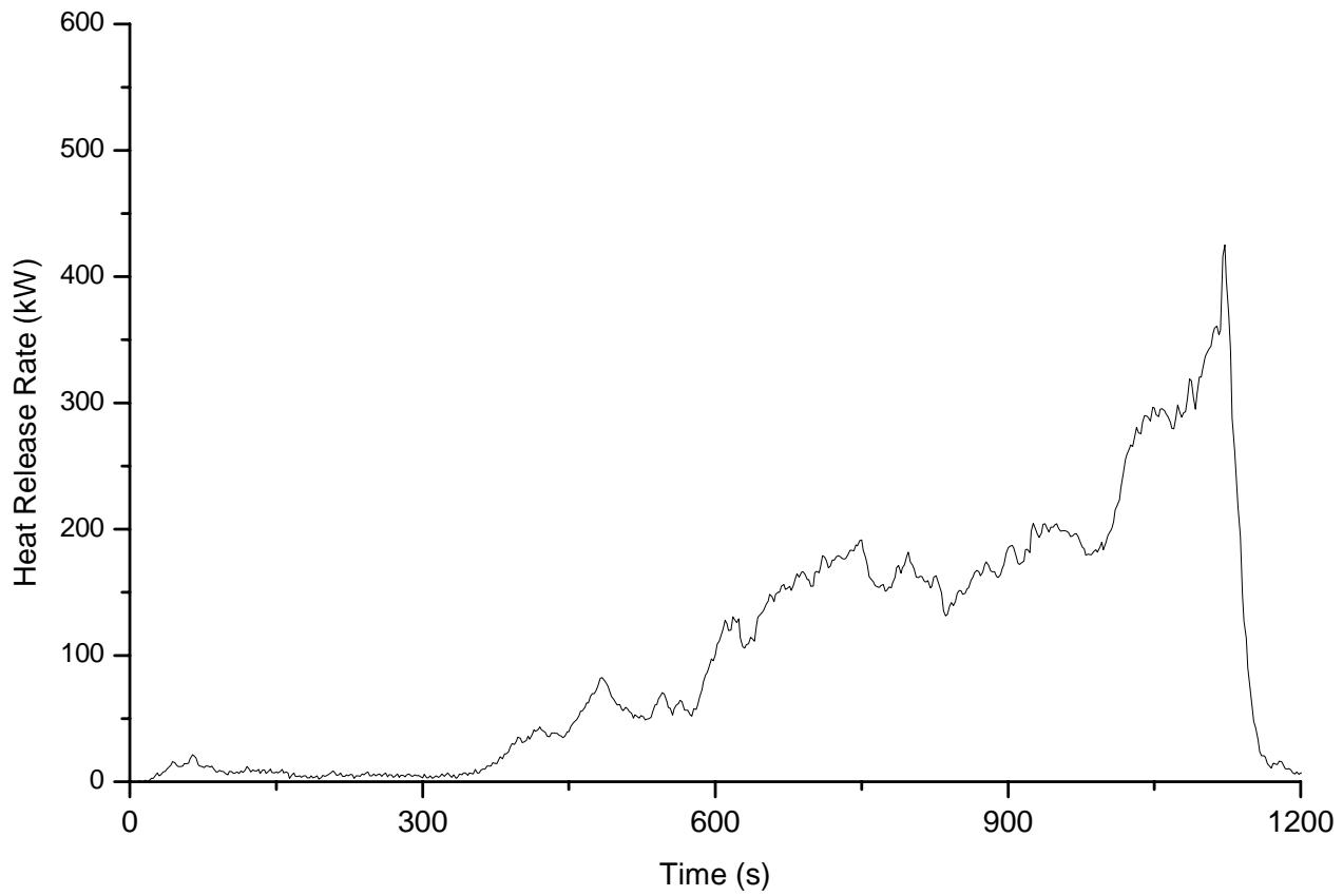
Figure 5I.3 – Heat Release Rate profile for Sofa fire (test terminated after 18½ mins)
