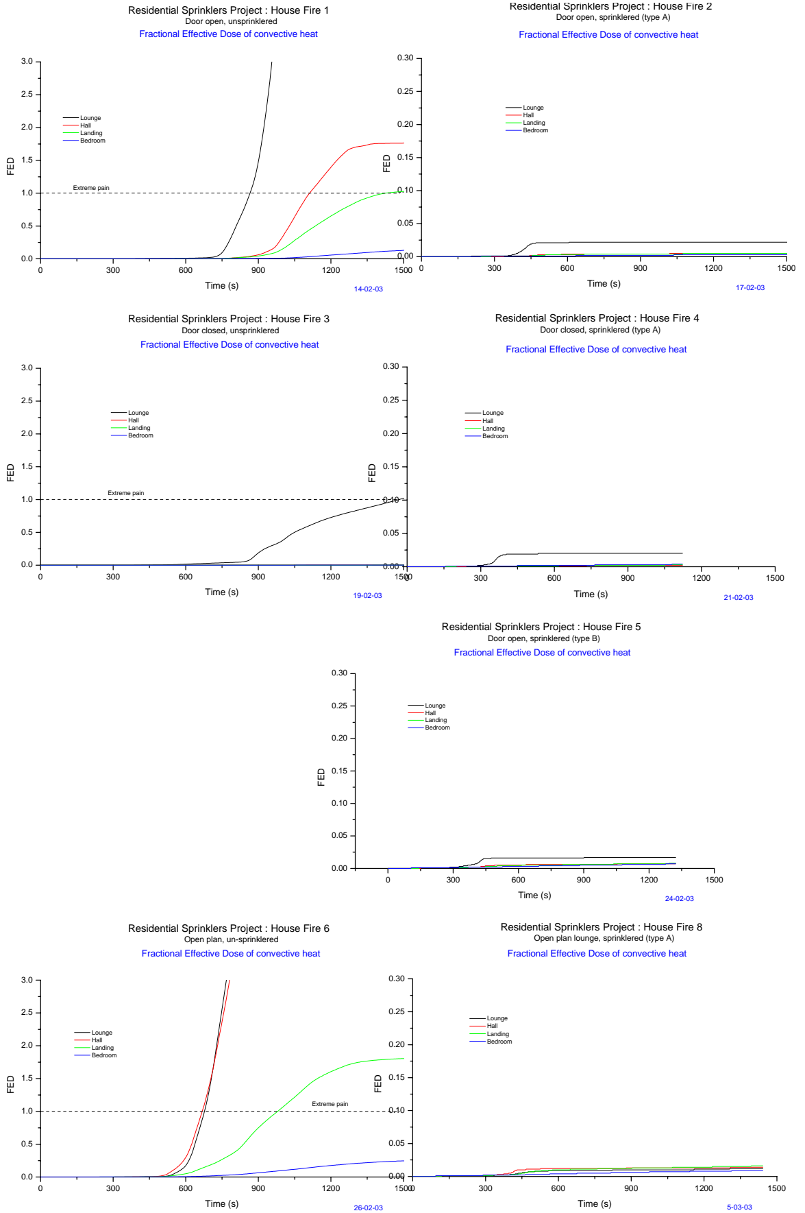
Figure 5D.3 House TV fires, FED due to convective heat in each room
