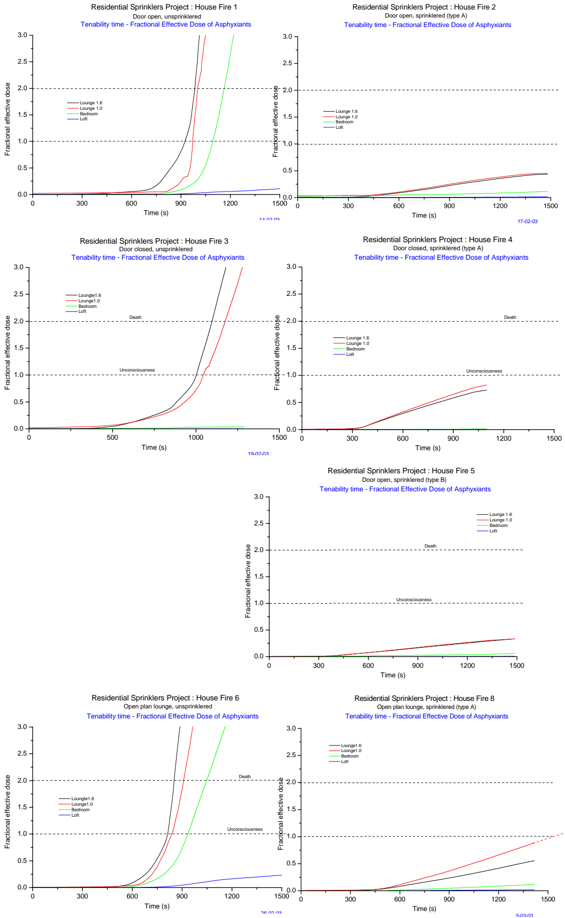
Figure 5D.2 House TV fires, FED due to asphyxiants gases in each room
