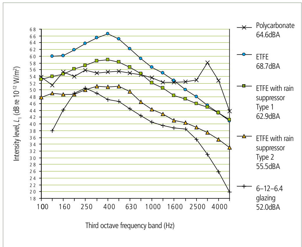
Figure 2 Measured sound intensity levels for the different roof elements.
