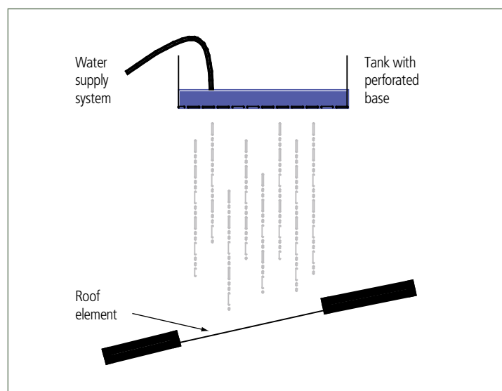
Figure 1 Test set-up - schematic diagram
